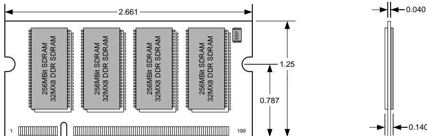
TSOP Package
