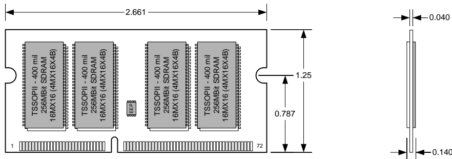
TSSOP Package
