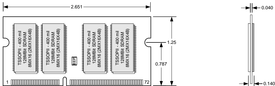
TSOP Package
